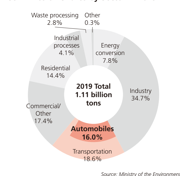
CO 2 Emission Shares by Sector in 2019
